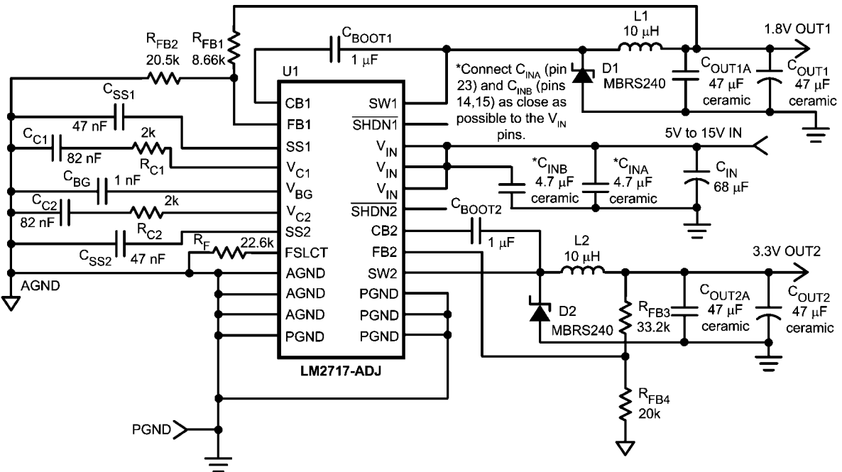
FIGURE 6. 3.3V, 1.8V Output Application
