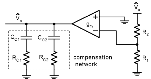
FIGURE 3. Compensation Network
